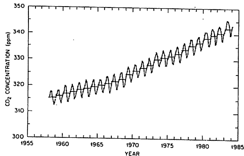
Figure 3.1. Atmospheric CO 2 in parts per million by volume (ppmv) concentrations at Mauna Loa Observatory, Hawaii. Measured amounts show seasonal fluctuations, primarily of biological origin, superimposed on an exponential growth. Source: C. Keeling, "Atmospheric CO 2 Concentration—Mauna Loa Observatory, Hawaii, 1958–1985," U.S. Department of Energy Report No. NDP-0011R1 (Oak Ridge, Tenn.: Carbon Dioxide Information Center, 1986).
